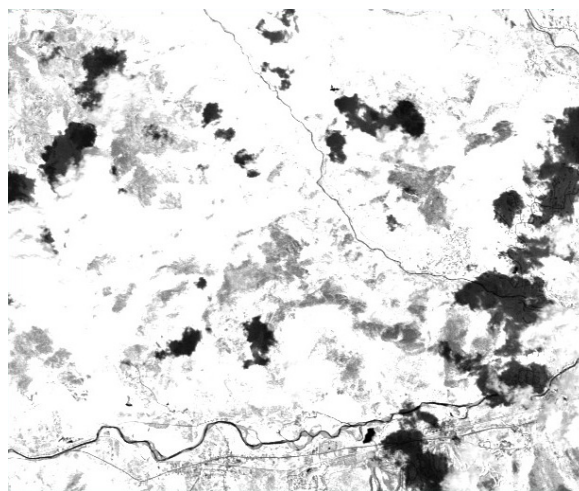
Figure 2. Retrieved shadow image for the White Mountains scene. The effect of ignoring the sky illumination of shadows (by setting c=0 ) is seen in Figure 5. In the visible the
