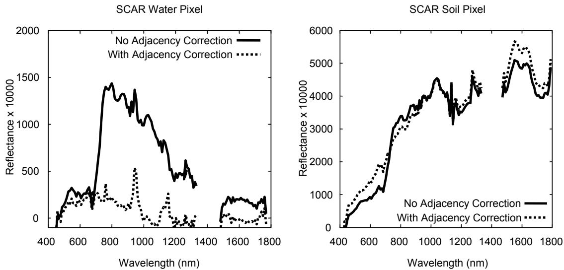
Figure 1. Comparisons of spectra retrieved by FLAASH from a very hazy 7/22/93 AVIRIS image of N. Carolina. The MODTRAN rural haze model was assumed
