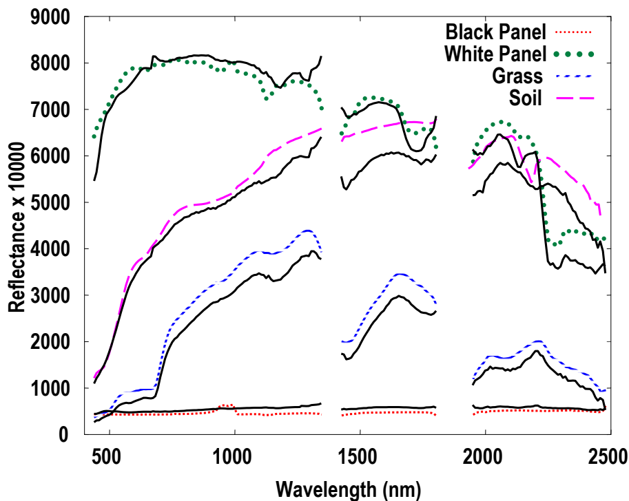
Figure 3. Comparison of ground truth spectra (dashed lines) and FLAASH retrievals from AVIRIS data (black lines) at Stennis Space Center using 1\text{ cm}^{-1} band model parameters, shifted wavelengths and spectral polishing ( N = 9 ).
