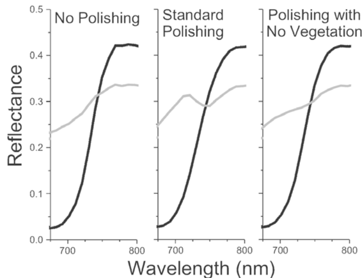
Figure 2. FLAASH retrieved spectra for soil (black curve) and vegetation (gray curve) in the chlorophyll edge region. At left, unpolished results; at center, with vegetation pixels included in the smooth set used to generate the polishing correction; and, at right, with vegetation pixels excluded from the smooth set.
